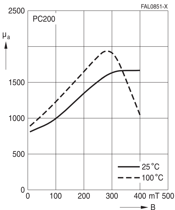
Amplitude permeability versus AC field flux density (measured on R34 toroids, f \leq 10 kHz)
