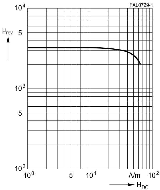
DC magnetic bias measured on RM cores (typical values) ( B \leq 0.25 \text{ mT} , f = 10 \text{ kHz} , T = 25 \text{ }^\circ\text{C} )
