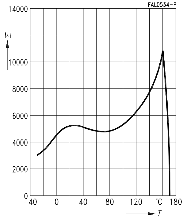
Initial permeability \mu_i versus temperature (measured on R29 toroids, B \leq 0.25 mT)
