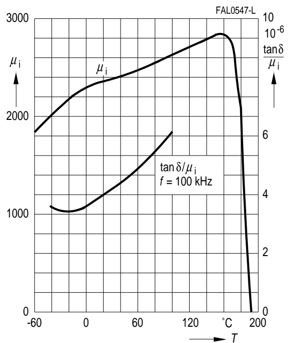
Initial permeability \mu_i and relative loss factor \tan \delta / \mu_i versus temperature (measured on R10 toroids, B \leq 0.25 mT)
