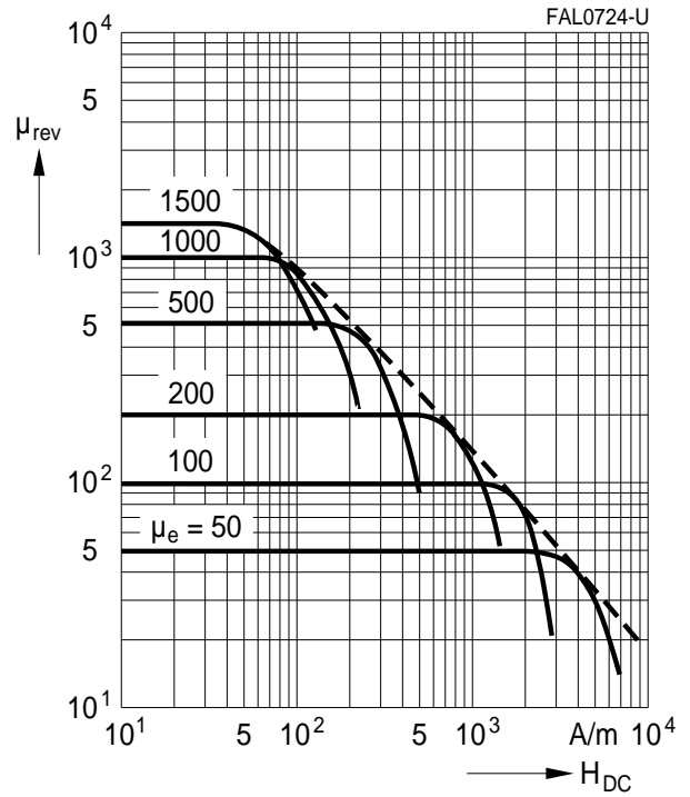
DC magnetic bias (measured on ETD cores, typical values) ( B \leq 0.25 mT, f = 10 kHz, T = 25 °C)
