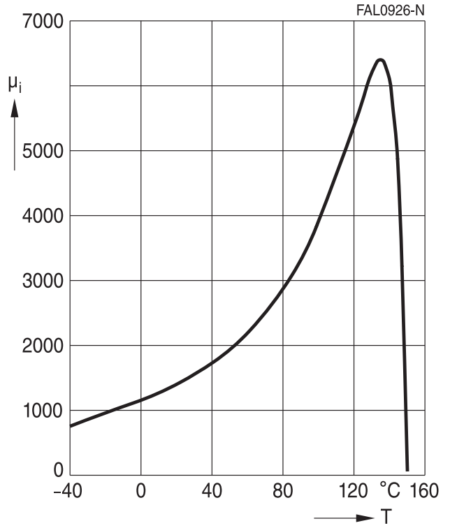
Initial permeability \mu_i versus temperature (measured on R12.5 toroids, \hat{B} \leq 0.25 mT)
