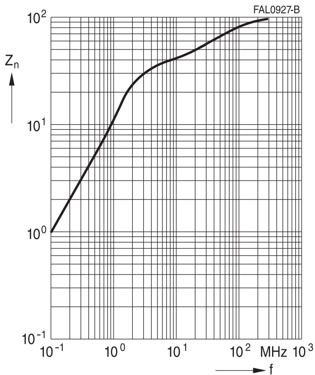
Normalized impedance of R12.5
