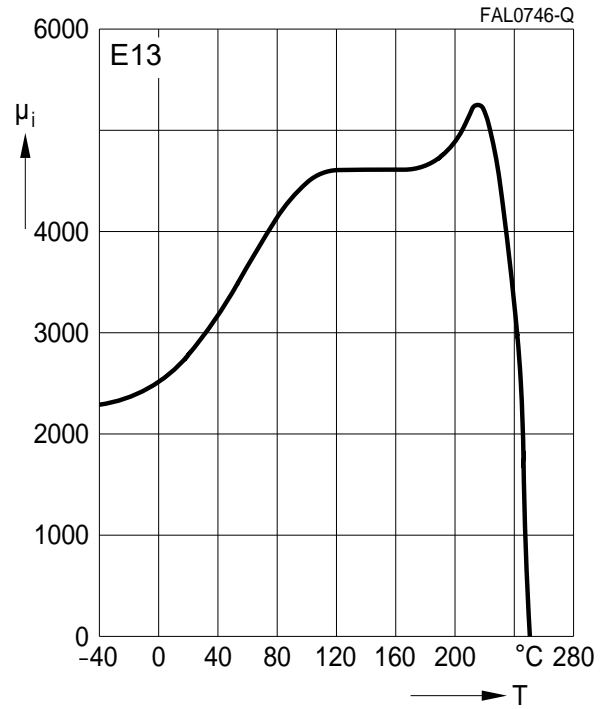
Initial permeability \mu_i versus temperature (measured on R34 toroids, B \leq 0.25 mT)
