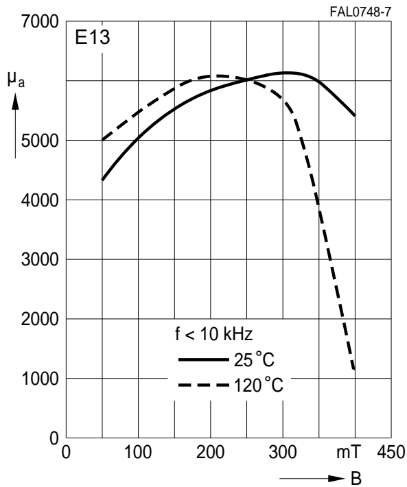
Amplitude permeability versus AC field flux density (measured on R34 toroids, B \leq 0.25 mT)
