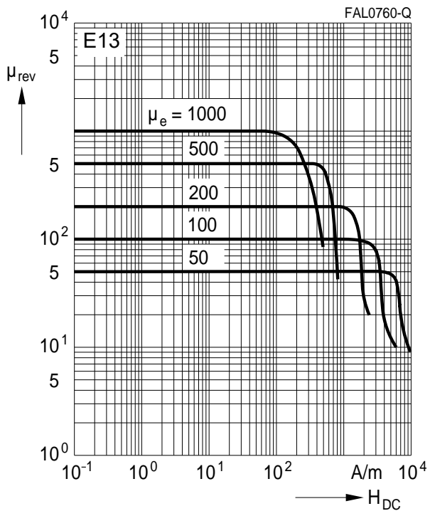
DC magnetic bias measured on ETD cores ( \hat{B} \leq 0.25 \text{ mT} , f = 10 \text{ kHz} , T = 25 \text{ °C} )
