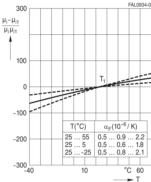
Permeability factor versus temperature (measured on P cores, \hat{B} \leq 0.25 mT), \mu_i \approx 1300
