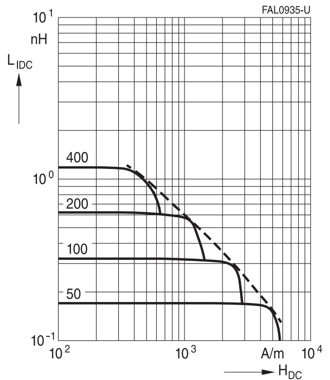
DC magnetic bias of P cores (typical values) \hat{B} \leq 0.25 mT, f = 10 kHz, T = 25 °C
