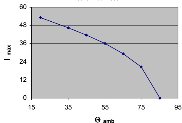
Max. allowable current (rms) at specific ambient Temp. B 25673A4302A080
