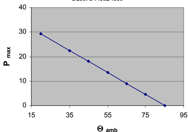
Max. allowable power loss at specific ambient Temp. B 25673A4302A080
