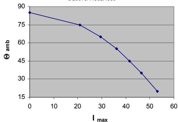
Max. allowable ambient Temp. at specific current (rms) B 25673A4302A080
