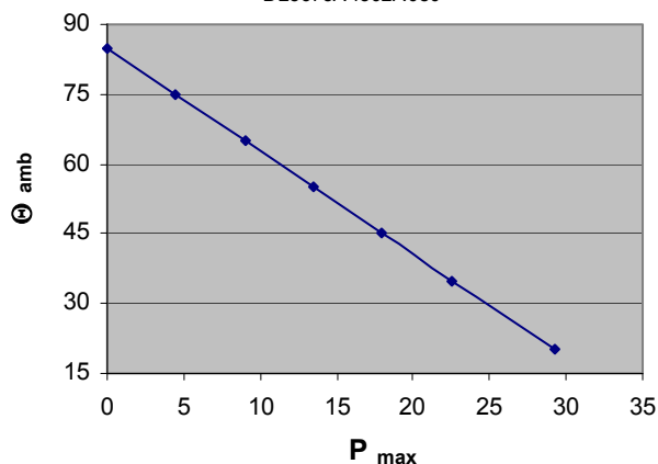
Max. allowable ambient Temp. at specific power loss B 25673A4302A080
