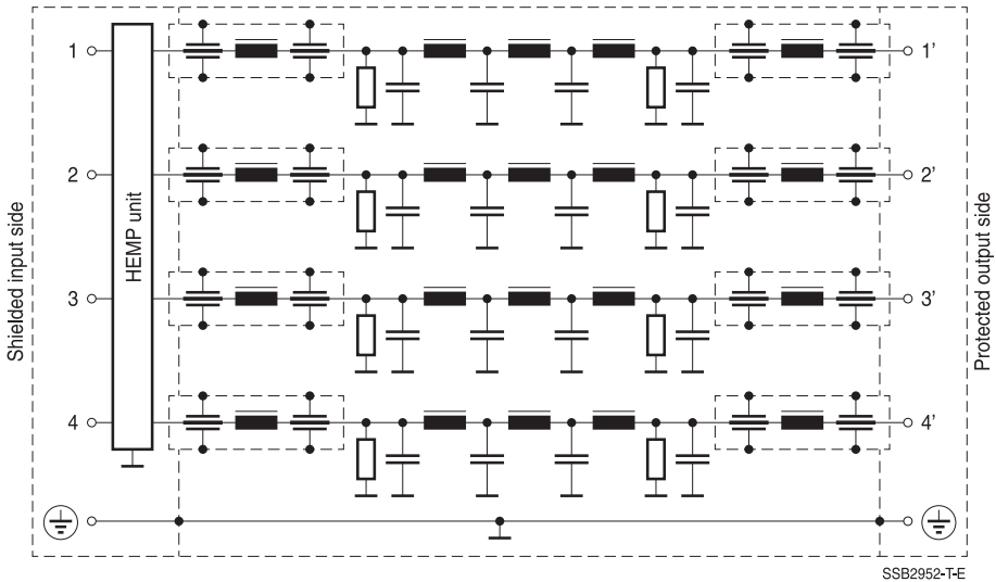
Circuit diagram 3: B84299C1251E313 (4 × 250 A), B84299D1251E313 (4 × 250 A)
