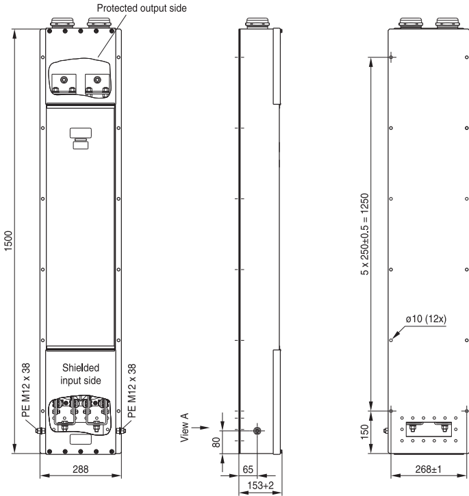
Drawing 8 – B84299D1501E313 (2 × 500 A) for assembly from inside to the shielded wall
