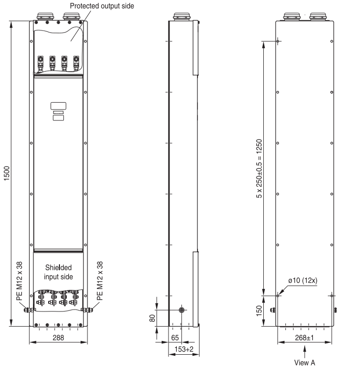
Drawing 5 – B84299C1251E313 (4 × 250 A) for assembly from inside to the shielded wall
