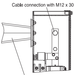
Connection of shielded input side
