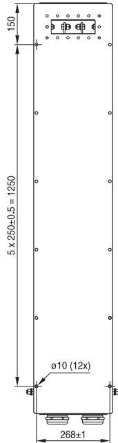
Drawing 2 – B84299D1251E303 (4 × 250 A) for assembly from outside to the shielded wall
