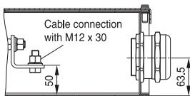
Connection of shielded input side
