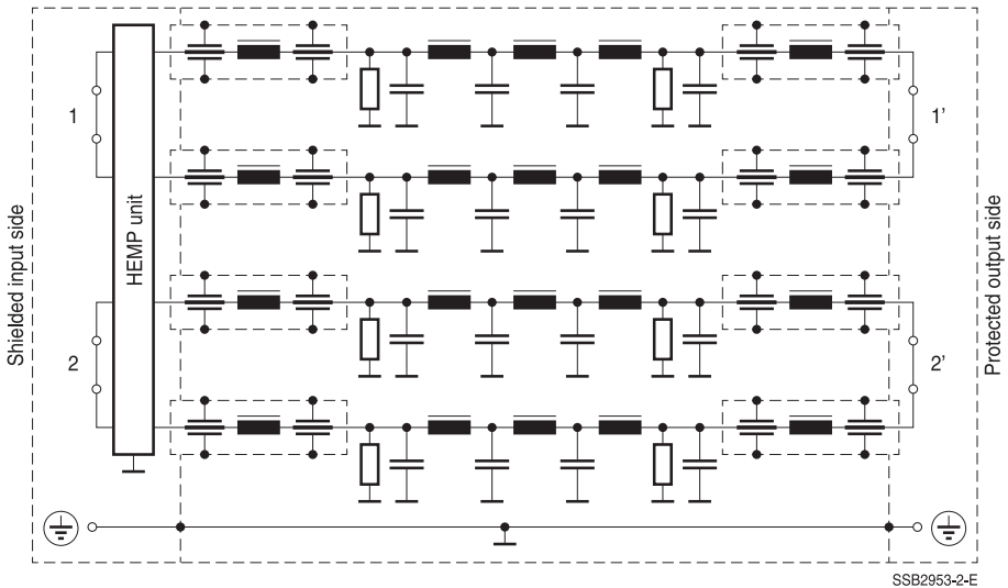
Circuit diagram 4: B84299C1501E313 (2 × 500 A), B84299D1501E313 (2 × 500 A)
