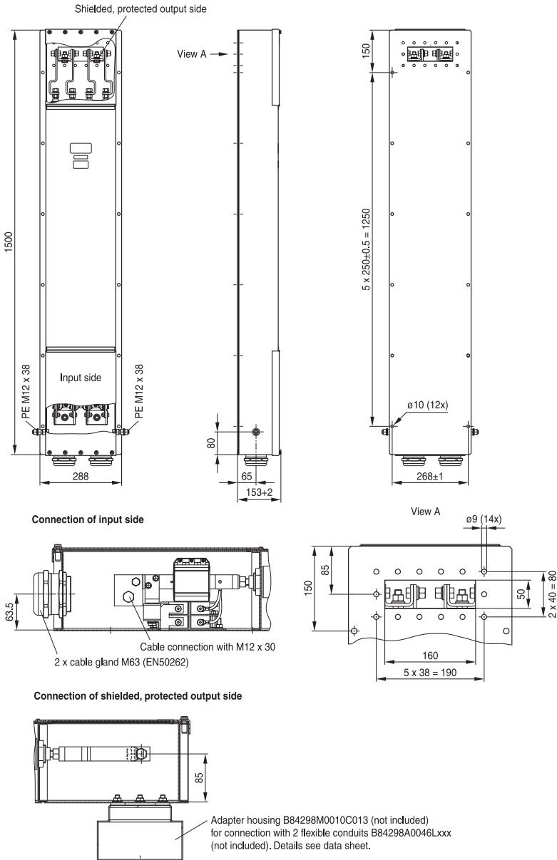
Drawing 4 – B84299D1501E303 (2 × 500 A) for assembly from outside to the shielded wall
