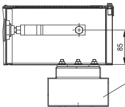
Connection of shielded, protected output side
