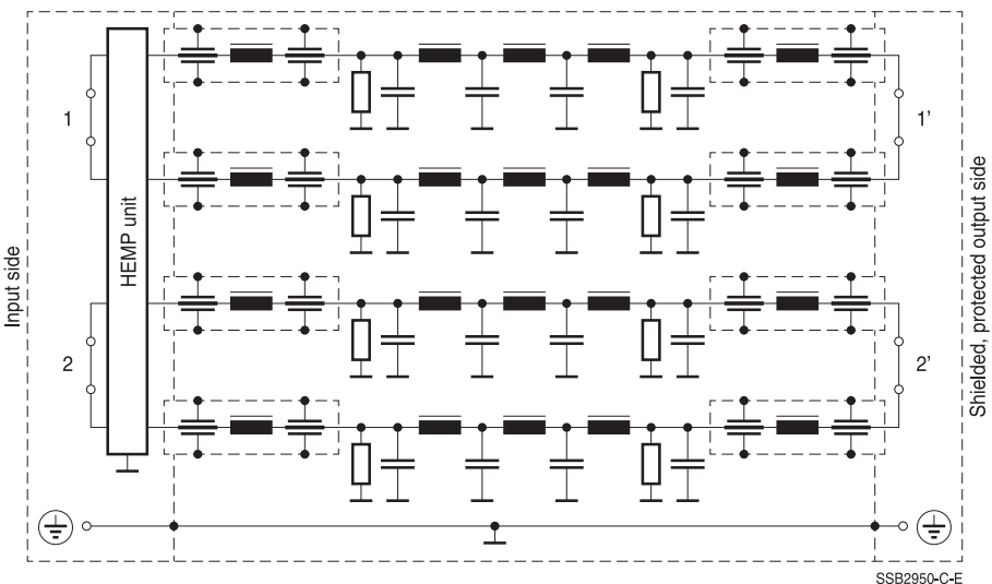
Circuit diagram 2: B84299C1501E303 (2 × 500 A), B84299D1501E303 (2 × 500 A)
