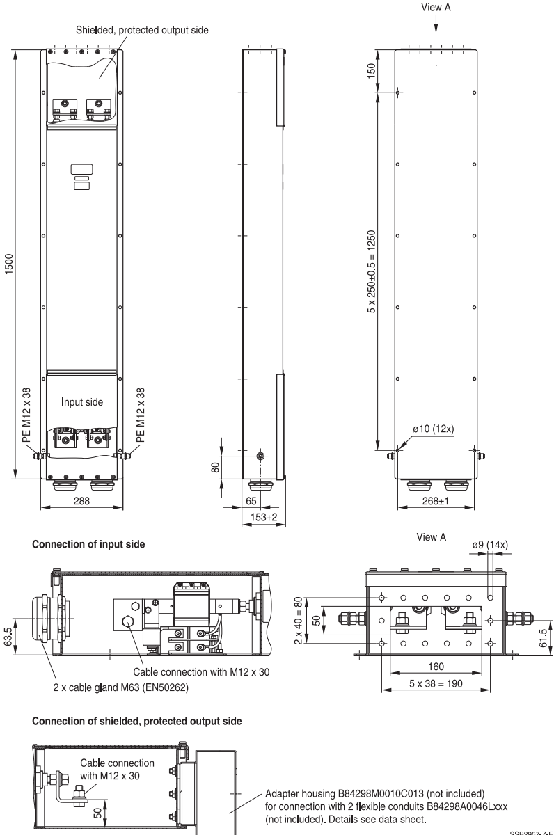
Drawing 3 – B84299C1501E303 (2 × 500 A) for assembly from outside to the shielded wall
