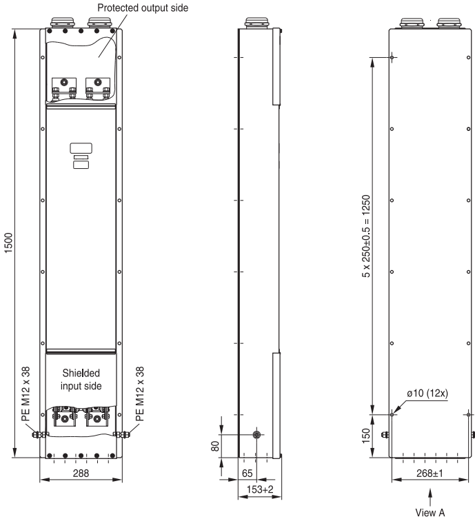
Drawing 7 – B84299C1501E313 (2 × 500 A) for assembly from inside to the shielded wall
