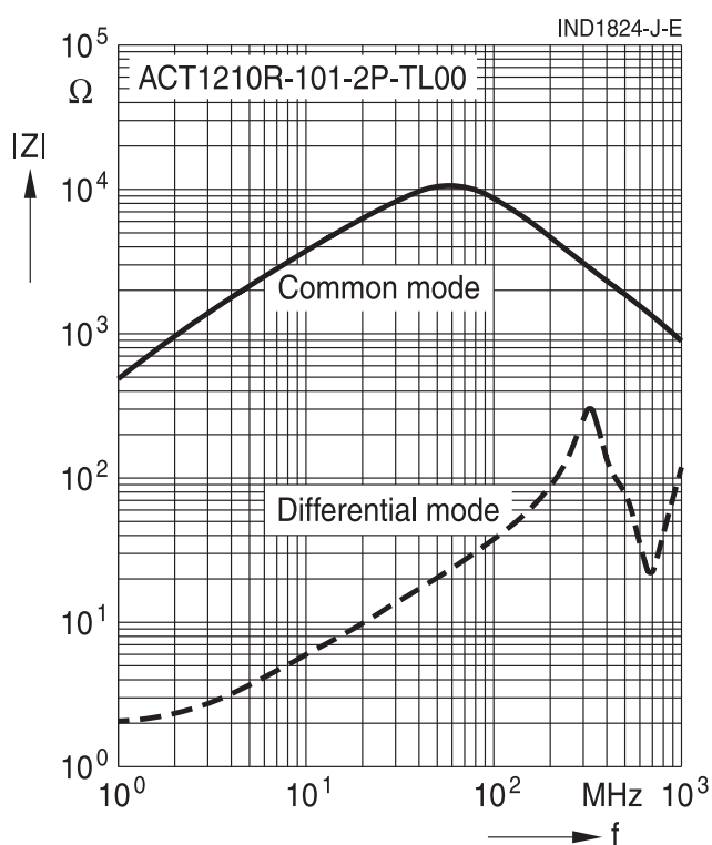
Impedance versus frequency (typical values) ACT1210R-101-2P-TL00
